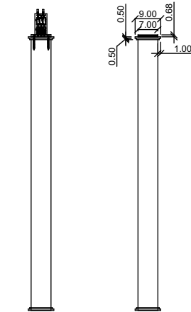
DETAIL PERSPECTIVE SCALE: 1/4" = 1'-0"
