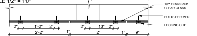
SINGLE POST- PLAN SCALE 1/2" = 1'0"
