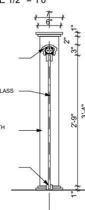
RAILING DETAIL- SECTION SCALE 1/2" = 1'0"
