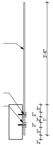
RAILING DETAIL- SECTION SCALE 1/2" = 1'0"
