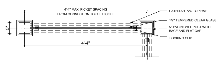
PVC POST CORNER SECTION- PLAN SCALE 1/2" = 1'0"
