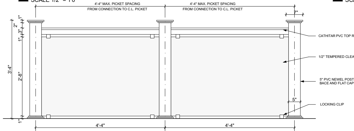
PVC POST CORNER SECTION- ELEVATION SCALE 1/2" = 1'0"
