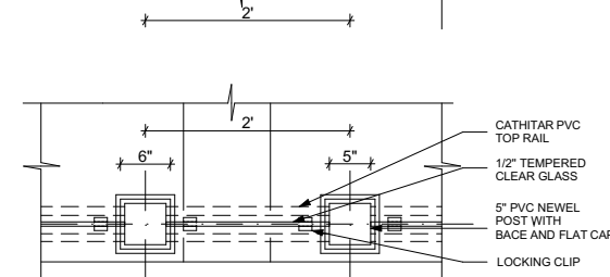
SINGLE POST- PLAN SCALE 1/2" = 1'0"
