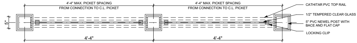
RAILING DETAIL- ELEVATION SCALE 1/2" = 1'0"
