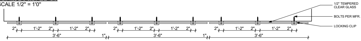
RAILING DETAIL- ELEVATION SCALE 1/2" = 1'0"
