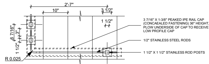
SINGLE POST- ELEVATION SCALE 1/2" = 1'0"
