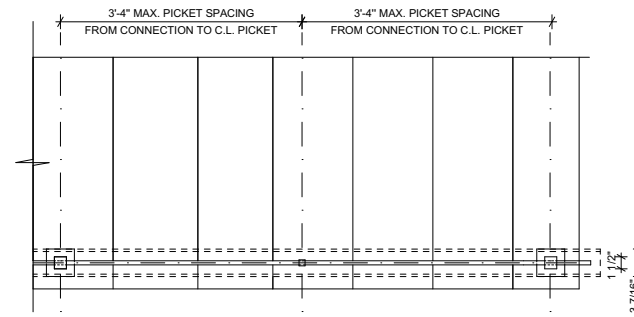
RAILING ON STAIRS- ELEVATION SCALE 1/2" = 1'0"
