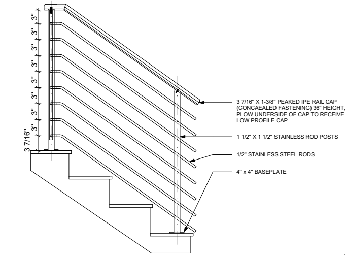
SINGLE POST- ELEVATION SCALE 1/2" = 1'0"
